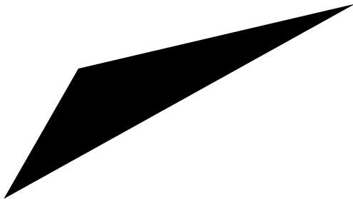
Wrong Triangle
