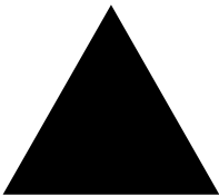
Regular Triangle
