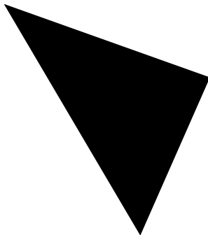
Irregular Triangle
