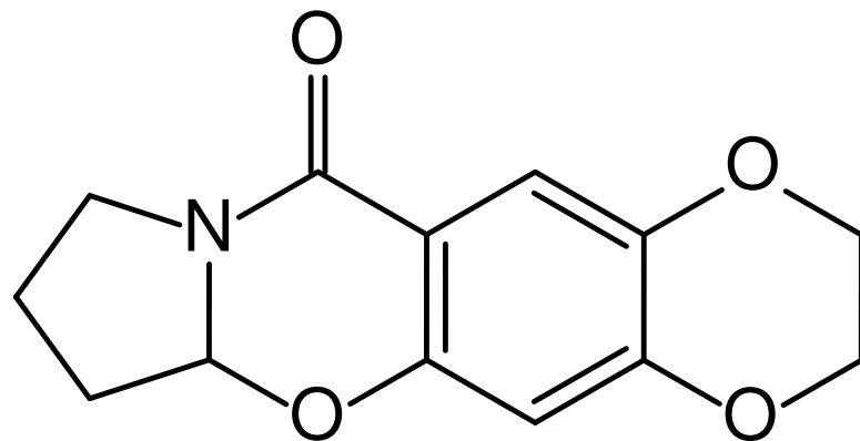
2H,3H,6aH-pyrrolidino[2'',1''-3',2']1,3-oxazino[6',5'-5,4]benzo[e]1,4-dioxan-10-one
