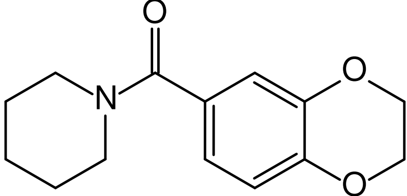
1-(1,4-benzodioxan-6-ylcarbonyl)piperidine
