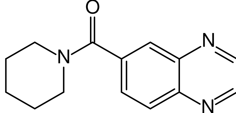
1-(quinoxalin-6-ylcarbonyl)piperidine
