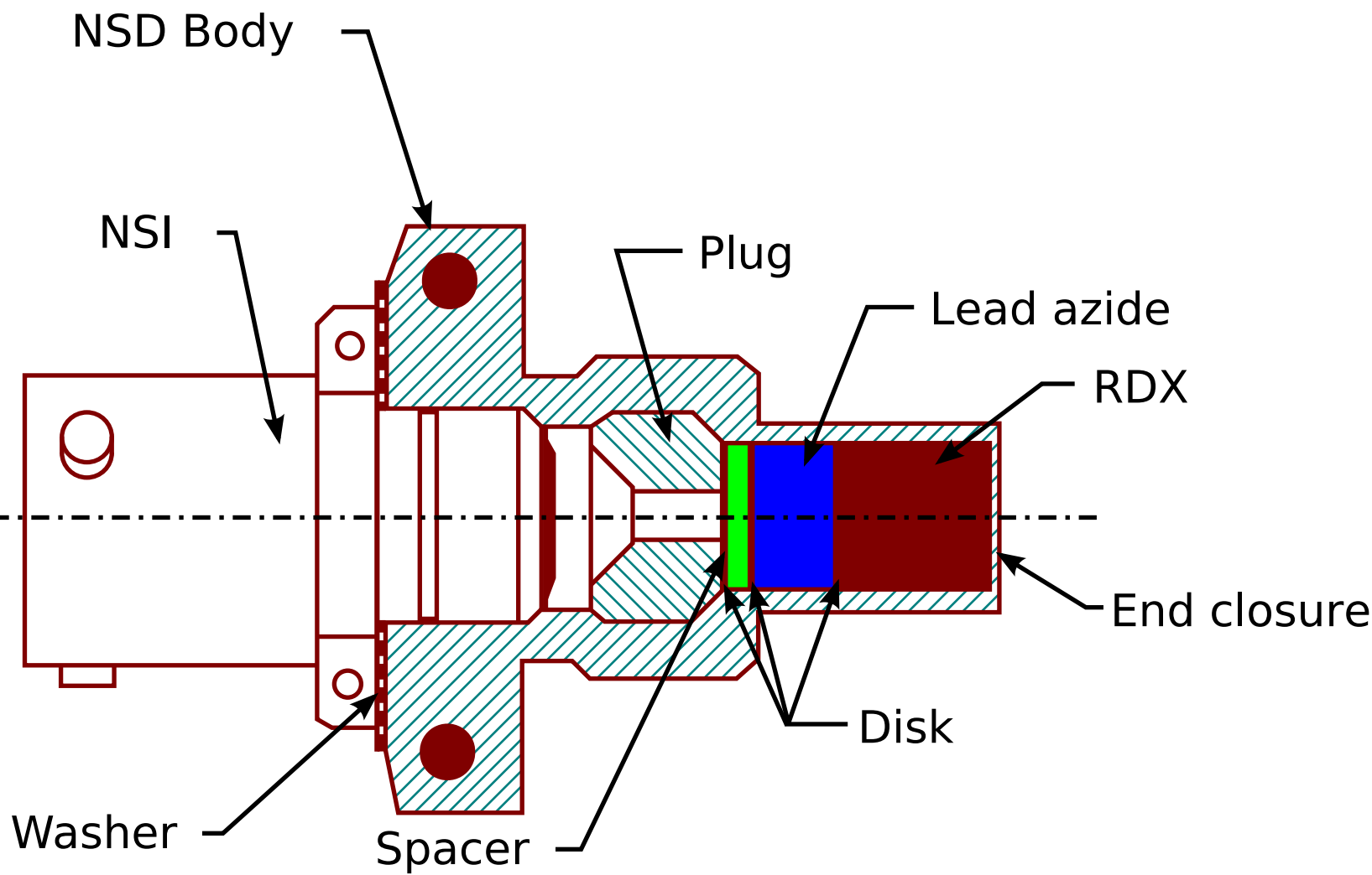
Schematic of NASA Standard Detonator
