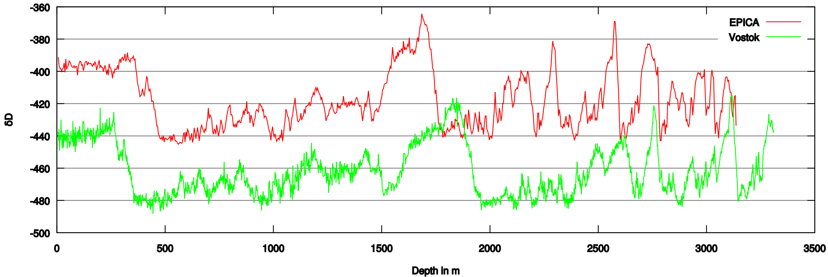
\delta D versus depth
