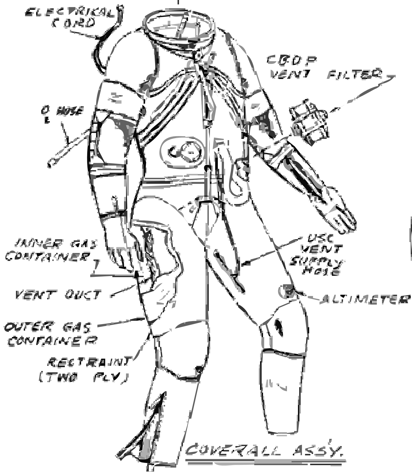
FIGURE 4 PROTOTYPE HIGH ALTITUDE FLYING OUTFIT SUBASSEMBLY ILLUSTRATION
