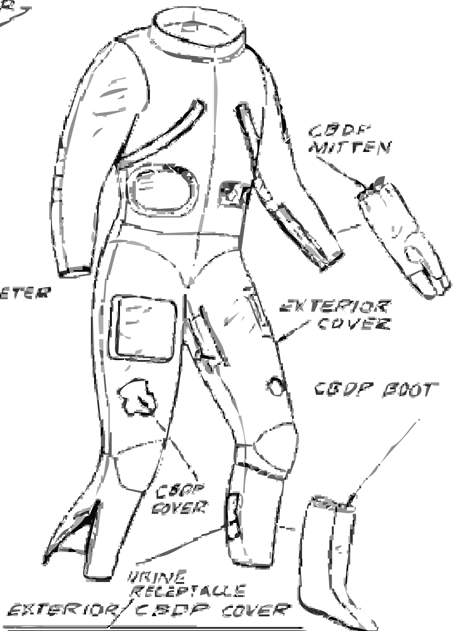
FIGURE 4 PROTOTYPE HIGH ALTITUDE FLYING OUTFIT SUBASSEMBLY ILLUSTRATION
