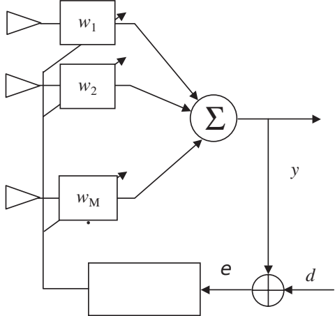
Smart Antenna
