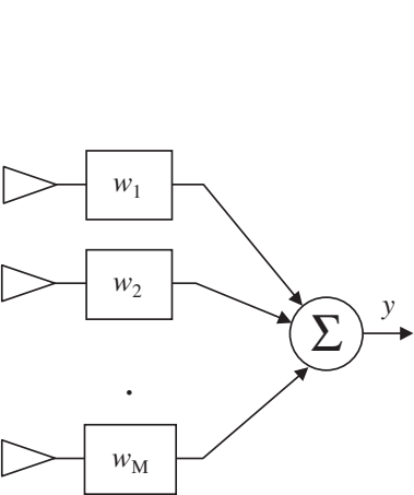
Traditional Array
