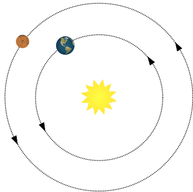
heliocentric system
