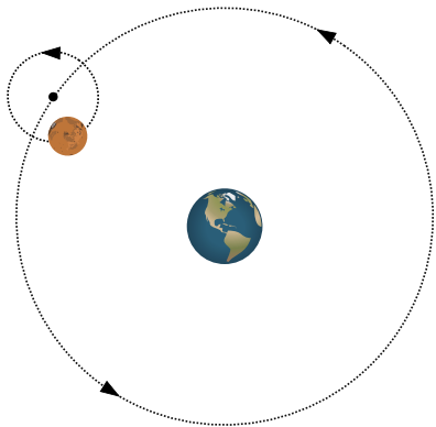
geocentric system
