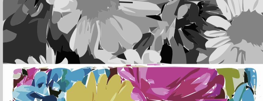
grayscale
