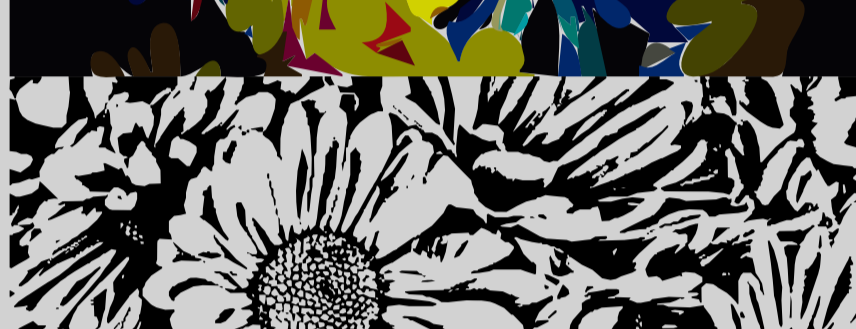
mapitize
