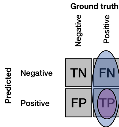
Recall
