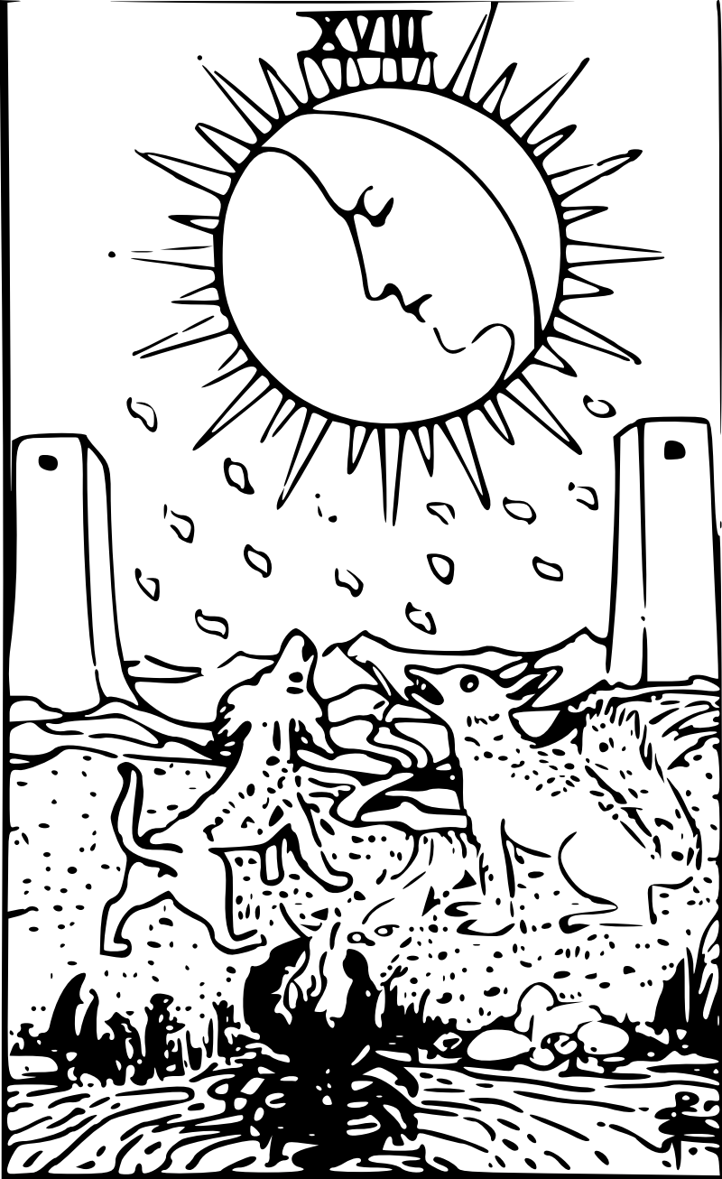
THE MOON.
